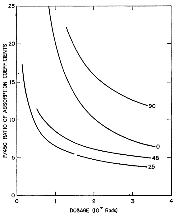
FIG. 4. The ratio of the absorption coefficients at the peaks of F center to that of the 450- \mu absorption bands as a function of gamma-ray dosage.
