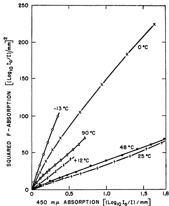
FIG. 5. The square of the absorption coefficient for the F peak plotted against the 450- \mu absorption coefficient for progressive irradiation of lithium fluoride at several temperatures indicated on the graph.
